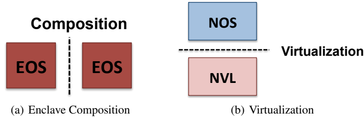
Fig. 5. Diagrams showing two key building blocks in the Hobbes design: (a) enclave composition, and (b) virtualization.
